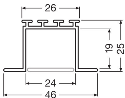
728412_FX-QMW-G1_TU26H25W10-300
